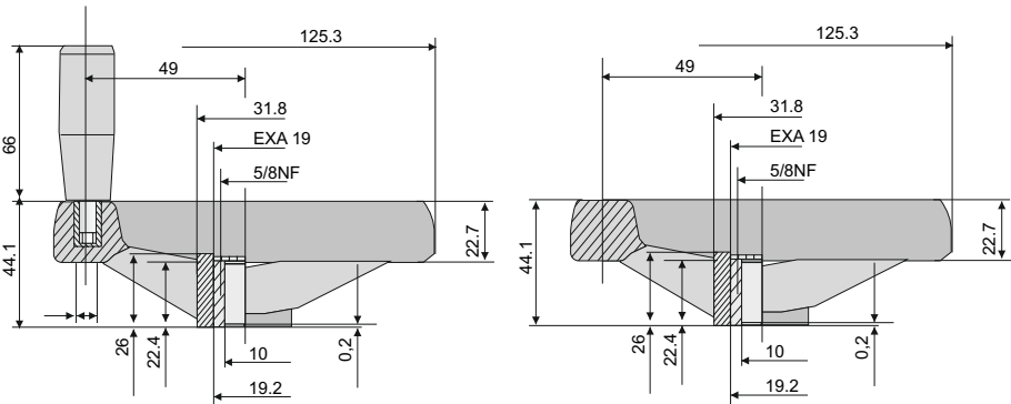
Volante Ø124 con Manija/sin Manija Steering Wheel Ø124 With Handle/Without Handle
