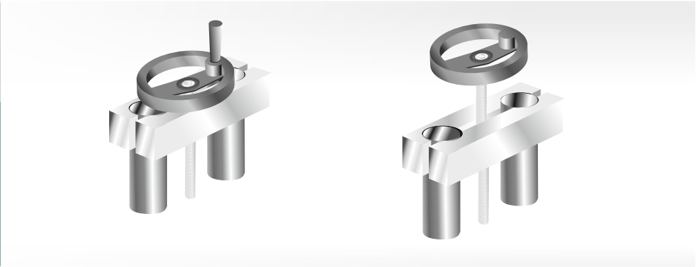
Volante Ø100 con Manija/sin Manija Steering Wheel Ø100 With Handle/Without Handle
